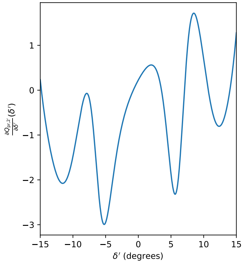
Angular derivatives at \lambda' = 1.00
