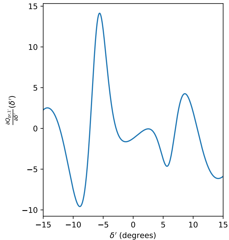
Angular derivatives at \lambda' = 1.00
